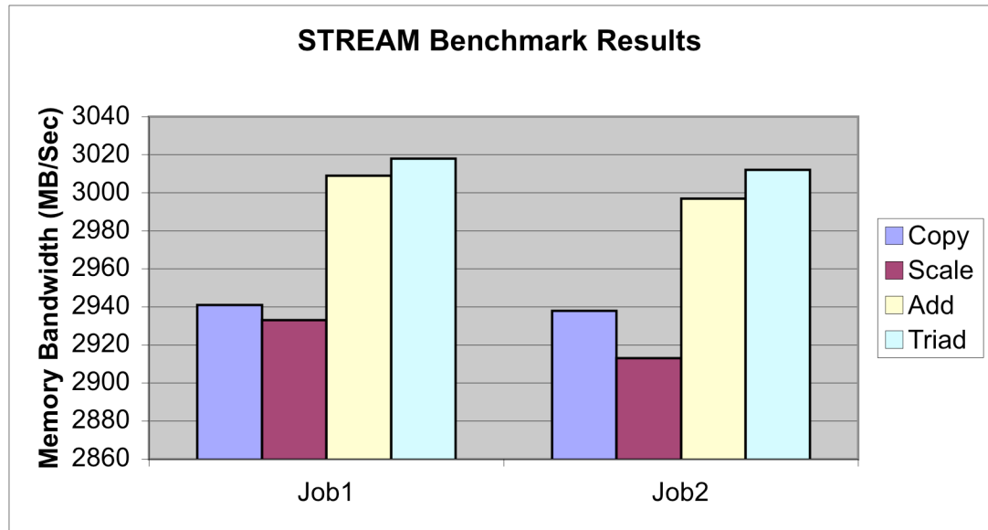
Figure 1. Bandwidth of two dual-core processors as determined by the STREAM benchmark.
